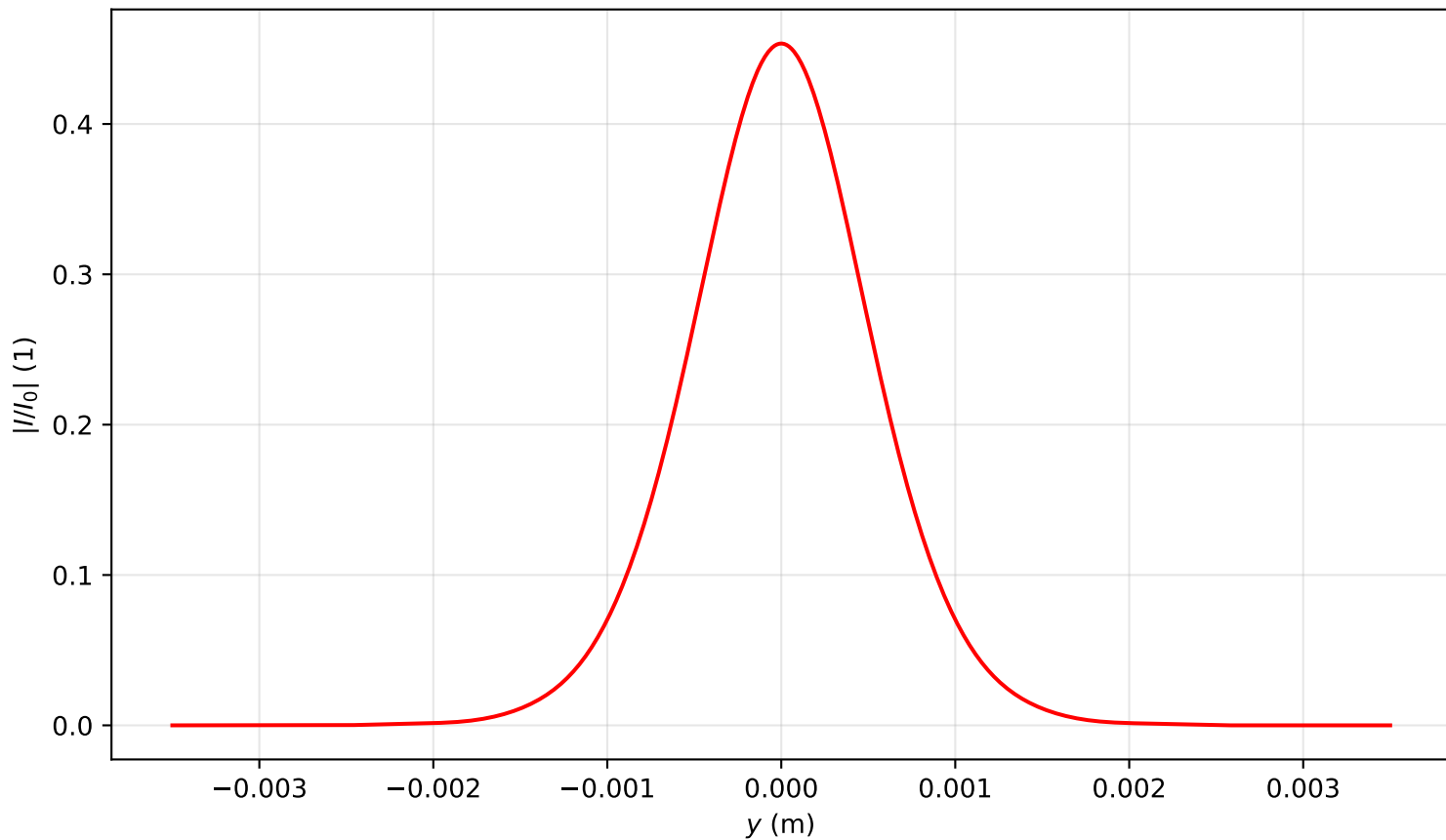
Intensity profile I(x = 0, y, z = 3.582)/I_0 , P_{in}=0.5P_{cr} , artificial time
